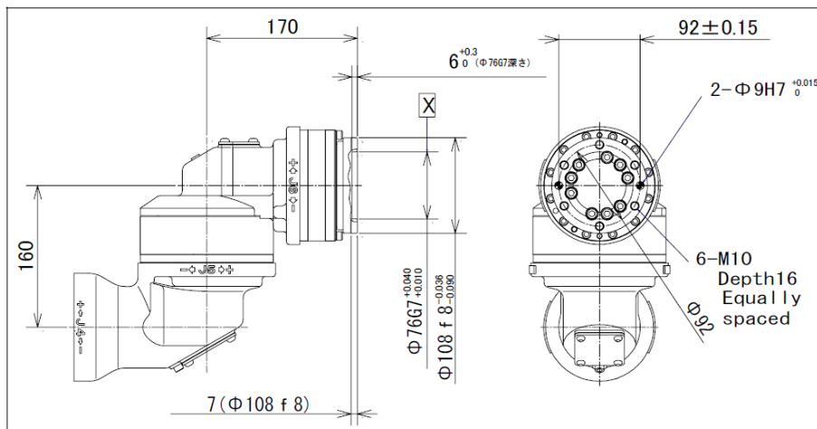
Fig.2.4 (e) End effector mounting face (Offset wrist, Special flange)
