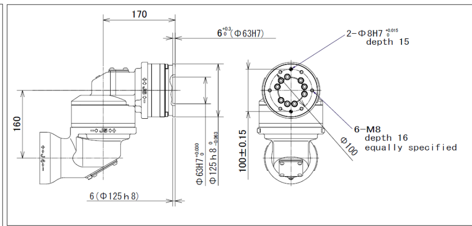
Fig.2.4 (f) End effector mounting face (Offset wrist, ISO flange)
